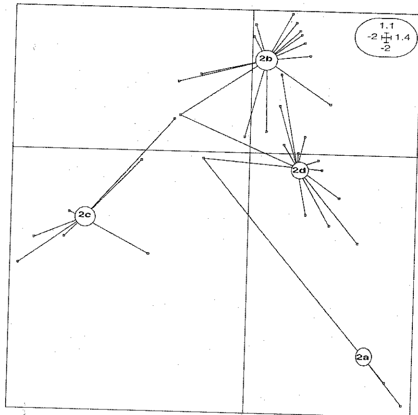
Fig. 3. Sample ordination by canonical correspondence analysis (CCA) with effect of the different decay stages of dead wood. 2a = Stage I, 2b = Stage II–III, 2c = stages V–VI–VII, 2d = mixed stages. Each circle is located at the barycenter of samples occurring in each category.
