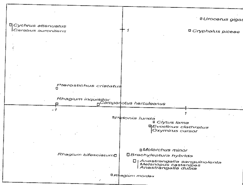
Fig. 4. Species ordination by canonical correspondence analysis (CCA) with additive effect of the decay stages of dead wood and management status.
